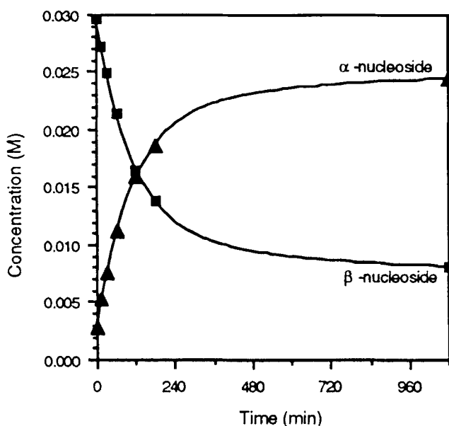
Figure 3. Anomerization of the -OTMS \beta -nucleoside (0.26 mmol) after warming from -30^{\circ}\text{C} to +21^{\circ}\text{C} . After complete reaction at -30^{\circ}\text{C} (1.75 hrs) the reaction vessel was placed in a +21^{\circ}\text{C} bath. Aliquots were removed at intervals, worked-up, and examined as in figure 1. (legend: \blacksquare = 3; \blacktriangle = 4)
