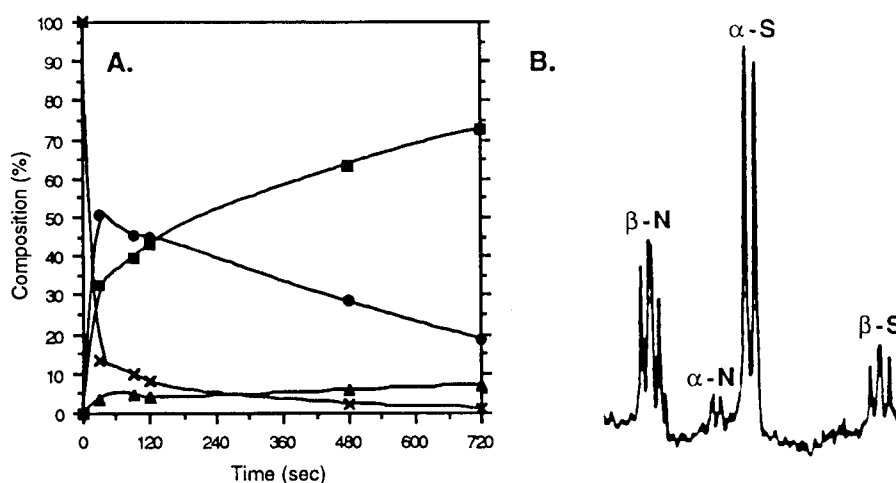
Figure 2. (A) Product composition vs. time after the addition of \text{SnCl}_4 to the \beta -S-glycoside intermediate (0.26 mmol). Aliquots were removed at intervals, worked-up, and examined as in figure 1. (legend: ■ = 3; × = 3a; ▲ = 4; ● = 4a) (B) Anomeric region of the ^1\text{H} NMR spectrum at t = 30 sec.
