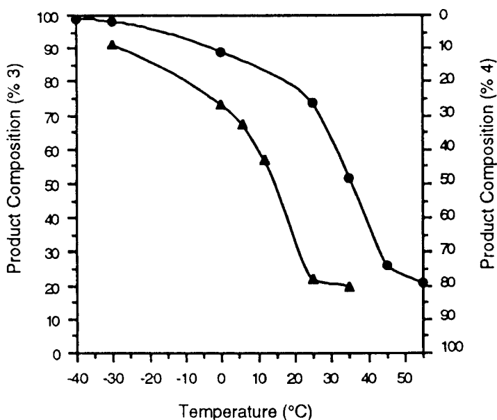
Figure 1. Anomeric product composition ( 3 & 4 ) as a function of temperature and solvent (legend: ● = \text{Cl}_2\text{CHCHCl}_2 ; ▲ = \text{ClCH}_2\text{CH}_2\text{Cl} ). Each data point represents a separate reaction (0.13 mmol) performed at the given temperature ( \pm 2^\circ\text{C} ). The compositions were determined by integrating the ^1\text{H} NMR signals of the crude reaction mixtures after work-up.
