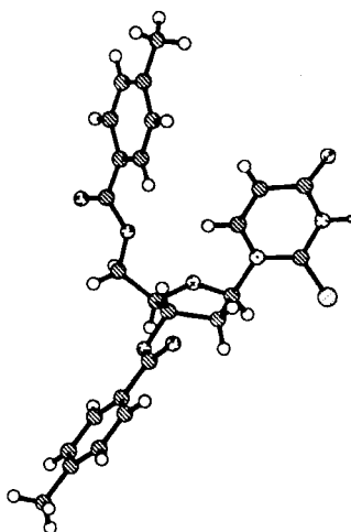
Figure 4. Single-crystal x-ray structure of the \beta -nucleoside 3 .
